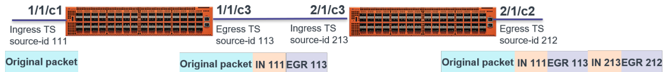
Figure 56 Timestamping
